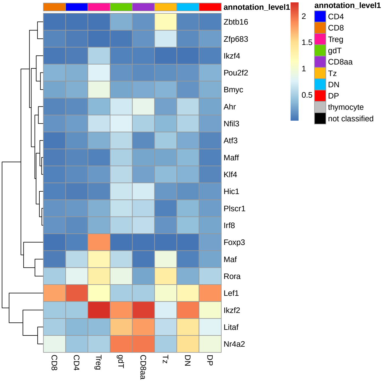
20 most lineage-specific TFs, log1p CP10K
